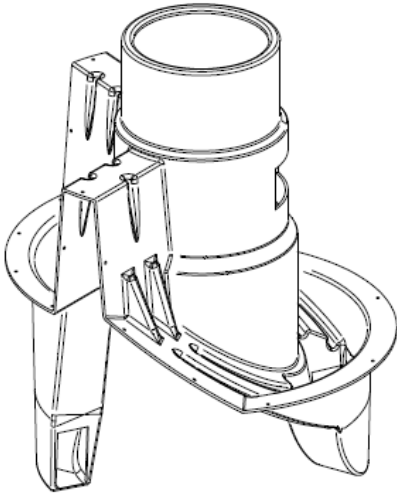
3 ft. First Defense HC ® Separation Module*
