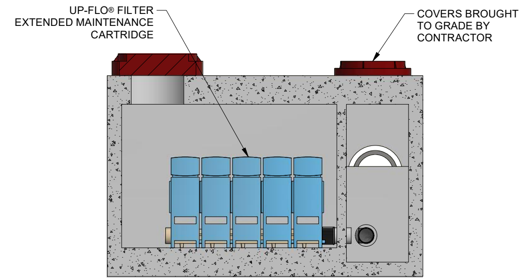
SECTION A-A ELEVATION VIEW
